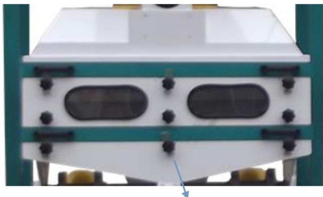
Through-hole handle to fasten sieves
